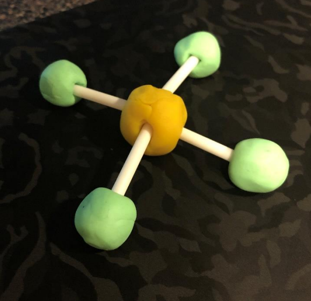
Sulfur Tetrafluoride
